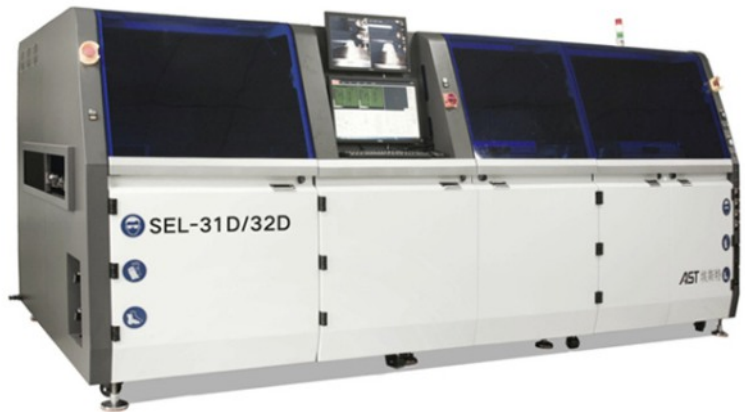
SEL-31D/32D IN-LINE DUAL POT SELECTIVE SOLDERING MACHINE
