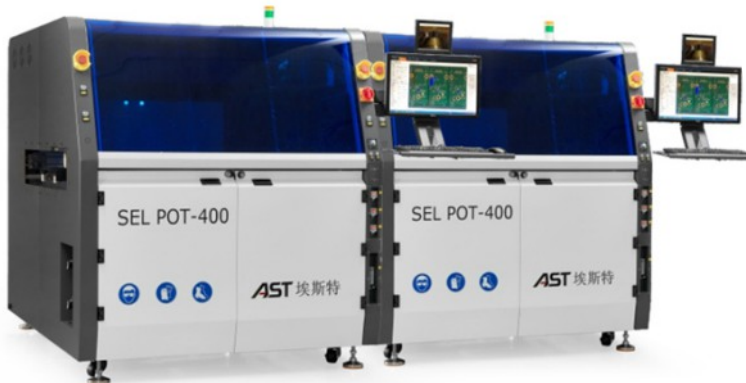
SEL POT-400 IN-LINE MODULAR SELECTIVE SOLDERING MACHINE
